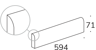
Skirting Battiscopa 60
